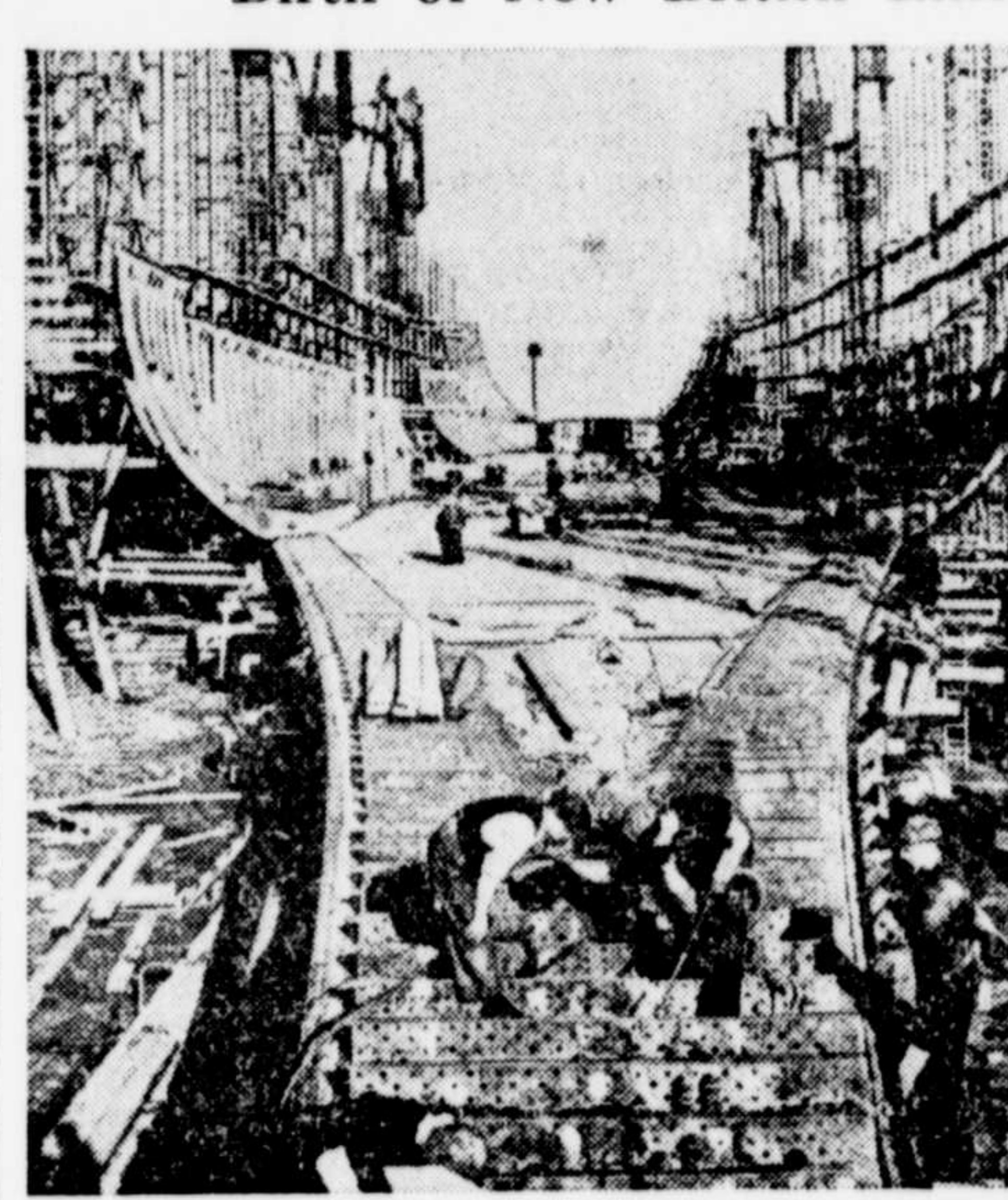
First photograph of the new 32,000-ton Cunard White Star liner, as yet known only as No. 1029, shows a view of the hull skeleton, looking toward the stern on the stocks of the shipyard at Birkenhead, England. This is the largest ship ever laid down in England.
