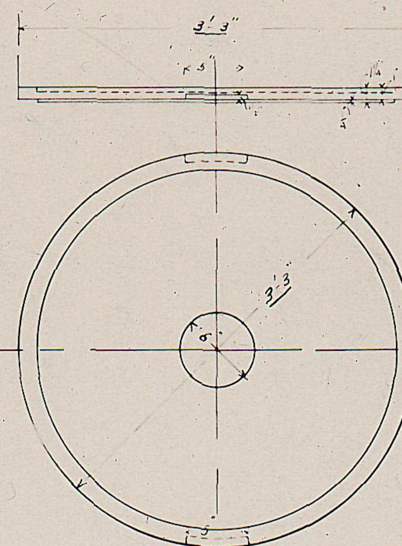
CAST IRON WEIGHT (20 REQUIRED)
